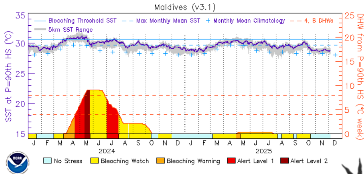
Coral Bleaching in Maldives during the season 2024
